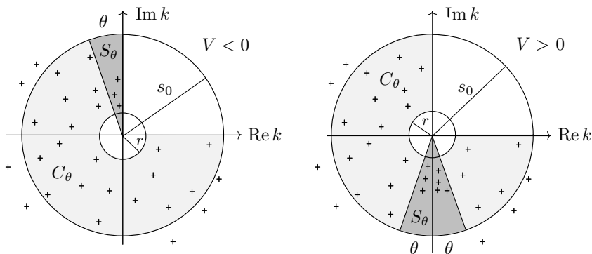
Figure 4.1. Resonances near a Landau level for V of definite sign. Resonances z = z_q(k) are concentrated near the semi axis k = -i(\text{sign } V)]0, +\infty[ . Moreover, for any \theta , the number of resonances in C_\theta is bounded by \mathcal{O}(|\ln r|) for s_0 = s_0(\theta) sufficiently small (Proposition 6). On the other hand, for any 0 < s_0 < \sqrt{2b} and any \theta , there is no resonance of H_0 + \varepsilon V in C_\theta for \varepsilon \leq \varepsilon_0(\theta) sufficiently small, and for compactly supported V we have a lower bound of the number of resonances in S_\theta (see Theorem 2).
