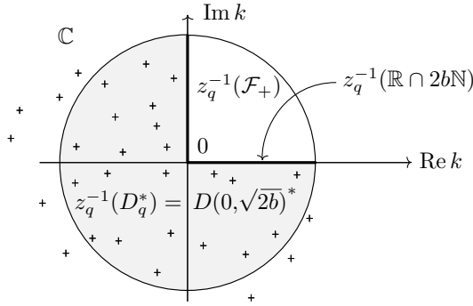
Figure 2.1. Pre-images under z_q
