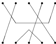
Figure 2.1. An element of P(5, 5) not in E(5, 5) .
