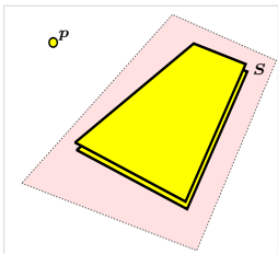
Base locus scheme \mathcal{B}(\mathcal{J}_{12}^5)
