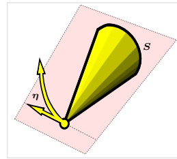
Base locus scheme \mathcal{B}(\mathcal{J}_5^5)
