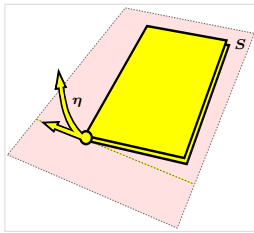
Base locus scheme \mathcal{B}(\mathcal{J}_3^5)
