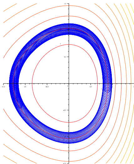
Figure 1.2. Numerical simulation of the flow of H when the magnetic field is given by B(x, y) = 2 + x^2 + y^2 + \frac{x^3}{3} + \frac{x^4}{20} , and \epsilon = 0.05 , t \in [0, 500] . The picture also displays in red some level sets of B .
