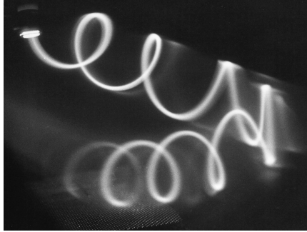
Figure 1.1. This photograph shows the motion of an electron beam in a non-uniform magnetic field. One can clearly see the fast rotation coupled with a drift. In the magnetic literature, the turning point (here on the right), due to the projection of the phase space motion onto the position space, is called a mirror point. Credits: Prof. Reiner Stenzel, http://www.physics.ucla.edu/plasma-exp/beam/BeamLoopyMirror.html
