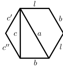
Figure 2.9. A hexagon in S , where d = b
