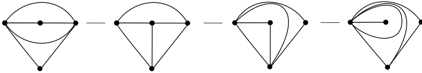
Figure 2.14. Modifying \gamma_0 to avoid a before u'
