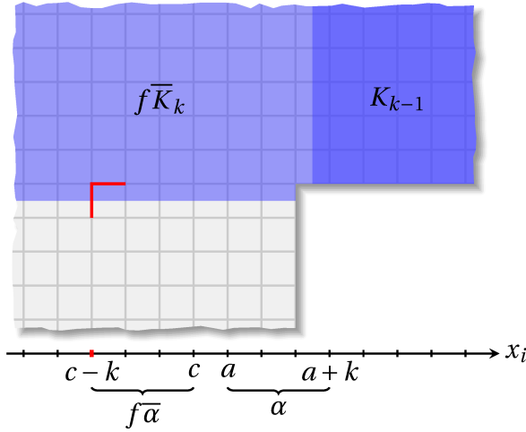
Figure 8.2. The elbow is aligned with the left endpoint of f\bar{\alpha} and the top side of the quadrant Q(K_{k-1}, f\bar{K}_k) . Hence f\bar{\alpha} is not to the right of \alpha . Since \alpha and f\bar{\alpha} cannot overlap, we have c \leq a . The elbow now generates a larger, “shifted” quadrant.
